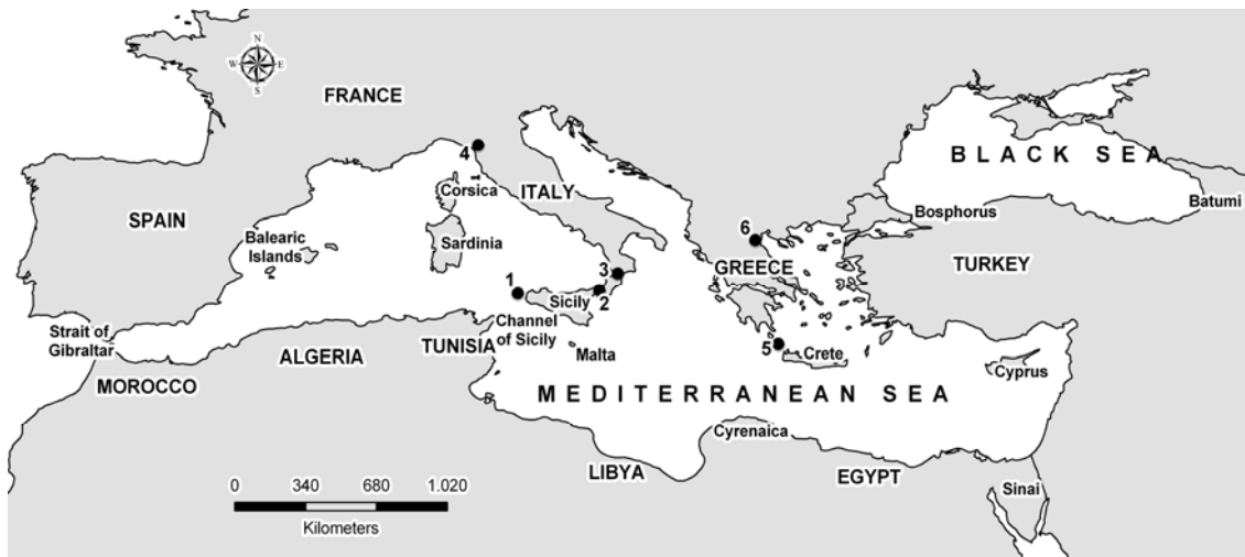
Fig. 2 The study area. The black dots indicate the fieldwork sites: 1) Marettimo island; 2) Strait of Messina; 3) Calabrian Apennines; 4) Apuan Alps; 5) Antikhitira island; 6) Mount Olympus.
